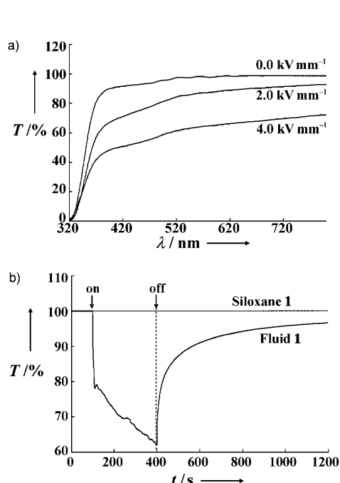
Figure 3. Changes in transmittance with dc field for BaTiO 3 particle/siloxane hybrid fluid. a) Change in transmittance of fluid 1 in dc fields of 0–4.0 kV mm -1 . b) Change in transmittance at 589 nm with on–off switching of a 4.0 \text{ kV mm}^{-1} dc field.
